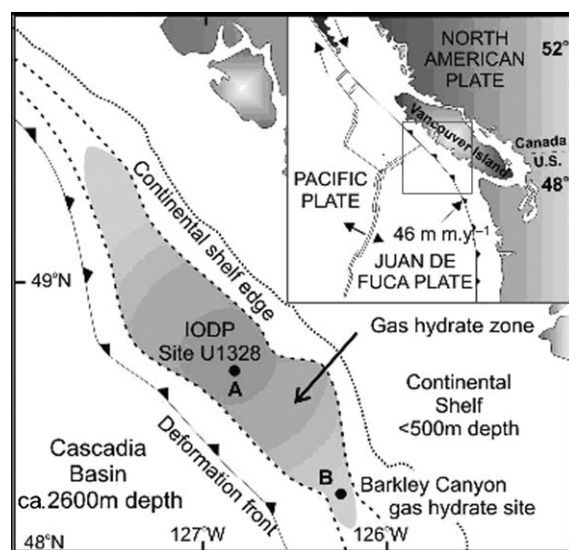
Figure 1. The locations of the studied samples (A, associated with a cold vent; B, associated with an oil seep); \text{m.y.}^{-1} refers to the moving rate of the Juan de Fuca plate in meters per thousand years.
